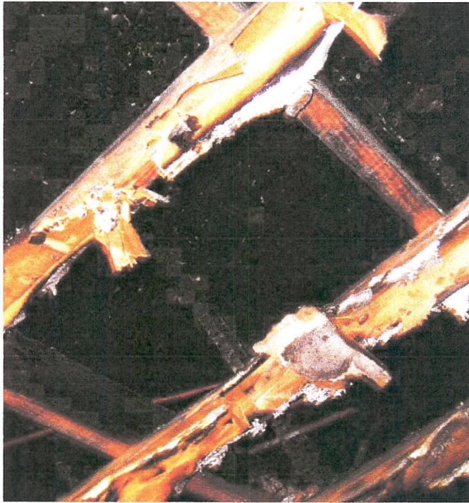
IMG_4308: Overview of interior damage.
